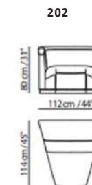
trapezoidal armless chair
