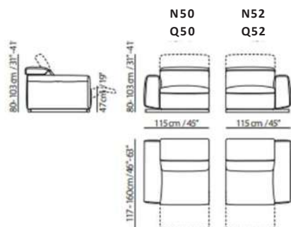
multi action power motion chair with arm
